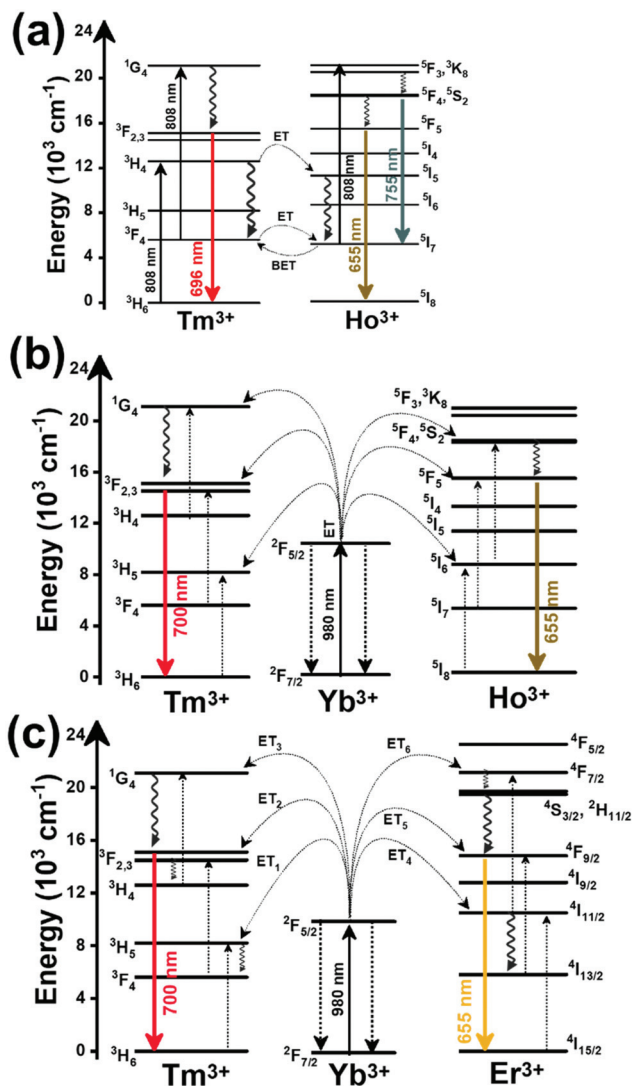
Fig. 9 Mechanisms of generation of the emission lines for: (a) Tm 3+ , Ho 3+ -doped KLu(WO 4 ) 2 nanocrystals after excitation at 808 nm, (b) Tm 3+ , Ho 3+ , Yb 3+ -doped YPO 4 or Gd 2 (WO 4 ) 3 nanoparticles after excitation at 980 nm, and (c) Tm 3+ , Er 3+ , Yb 3+ :YF 3 nanoparticles embedded in a glass ceramic after excitation at 980 nm.
