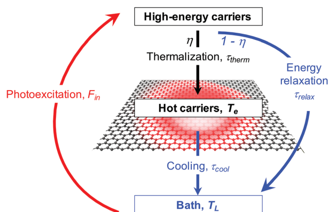
Fig. 3 Schematic illustration of the formation of hot carriers via photo-excitation, followed by thermalization of high-energy carriers. Since high-energy carriers can also directly relax to their environment, the branching ratio between these two processes determines the heating efficiency \eta .
