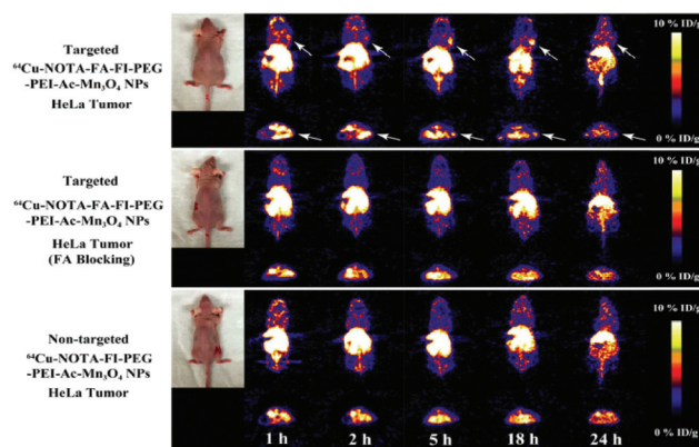
Fig. 8 MicroPET images of nude mice bearing HeLa xenografted tumors at different time points post-intravenous injection of the ^{64}\text{Cu} -NOTA-FA-Fl-PEG-PEI-Ac- \text{Mn}_3\text{O}_4 NPs (targeted NPs), ^{64}\text{Cu} -NOTA-FA-Fl-PEG-PEI-Ac- \text{Mn}_3\text{O}_4 NPs with FA blocking, and ^{64}\text{Cu} -NOTA-Fl-PEG-PEI-Ac- \text{Mn}_3\text{O}_4 NPs (nontargeted NPs). The whole-body coronal (top) and transverse (bottom) microPET images of nude mice bearing HeLa xenografted tumors are shown. Tumors are indicated by arrows. Reprinted with permission from ref. 169 Zhu et al. , ACS Appl. Mater. Interfaces , 2018, 10, 34954–34964. Copyright©2018, the American Chemical Society.
