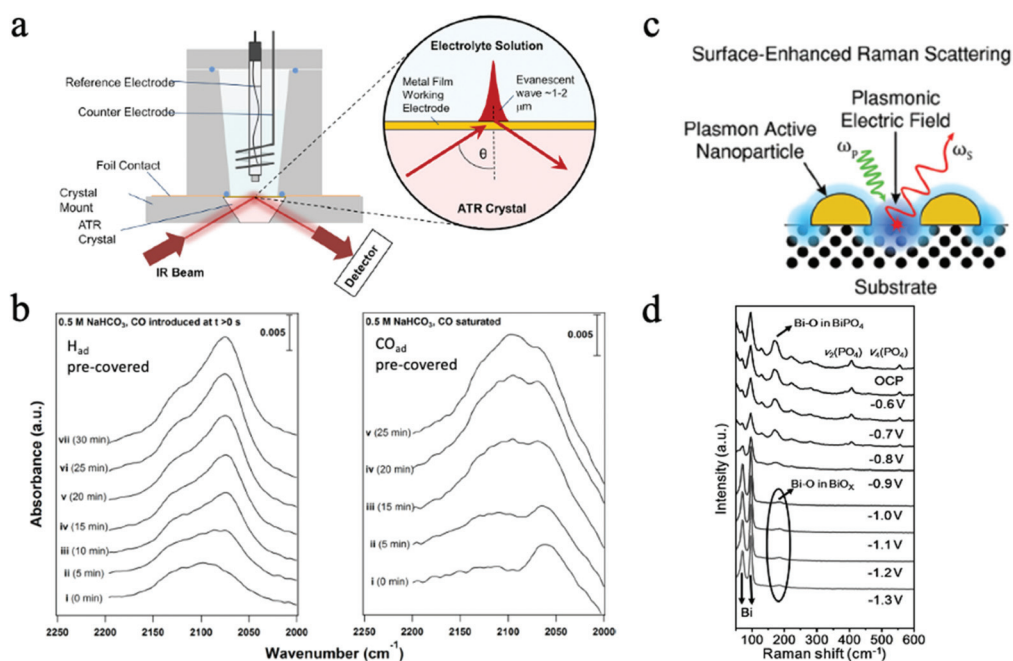
Fig. 10 (a) Mechanism of in situ ATR. Copyright 2017, crown; (b) time-resolved SEIRA spectra of \text{H}_{\text{ad}} accumulation on CO-adsorbed Cu surface. Copyright 2016, American Chemical Society (c) mechanism of SERS. Copyright 2021, Royal Society of Chemistry; (d) operando Raman spectra under different applied potential. All panels reproduced with permission. 198–201 Copyright 2021, 2021 Wiley and Sons.
