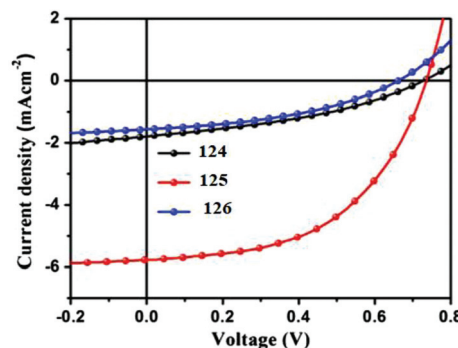
Fig. 22 Current–voltage characteristics of optimized photovoltaic cells based on 124 : PC 61 BM, 125 : PC 61 BM and 126 : PC 61 BM under illumination of AM 1.5, 100 \text{mW cm}^{-2} white light. Reproduced with permission of Elsevier. 74
