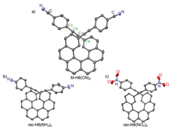
Fig. 2. X-ray crystallographic views of M -H6(CN) 2 , rac -H6(NH 2 ) 2 , and rac -H6(NO 2 ) 2 (only one enantiomer is shown). P 4 1 2 1 2 , P 2 1 / c and C 2 / c space groups for M -H6(CN) 2 , rac -H6(NH 2 ) 2 , and rac -H6(NO 2 ) 2 , respectively.
