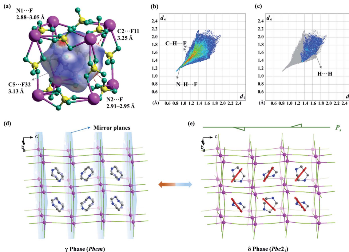
Fig. 7 (a) Hirshfeld surfaces mapped with d_{\text{norm}} over the range of -0.50 (red) to 0.90 (blue) for the guest cation at the \delta phase. Fingerprint plot for H \cdots F contacts (b) and H \cdots H contacts (c) of guest cations at the \delta phase. Crystal structures at 338 K ( \gamma phase, d) and 293 K ( \delta phase, e) along the diagonal of the (001) lattice plane. For clarity, H atoms are omitted. In the \gamma phase, the organic cations are located in two sites about the mirror planes (light blue planes). In the \delta phase, the orientations of ordered organic cations (the directions of dipole moment are shown in red arrows) induce spontaneous polarization along the c -axis and the disappearance of the mirrors in the \delta phase.
