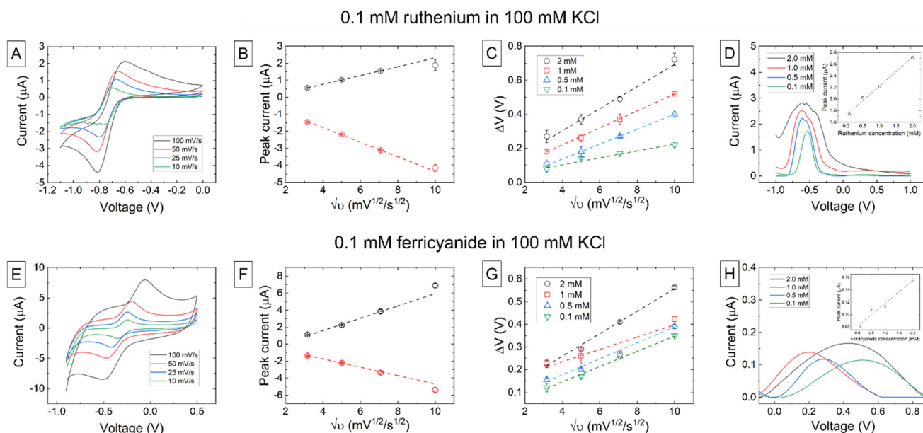
Fig. 3 (A) and (E) CV measurements of HexRu and FC, respectively, in 100 mM KCl at increasing scanning rates of 10, 25, 50, and 100 mV s -1 . (B) and (F) Oxidation and reduction peak currents against the square root of the scan rate for each mediator. Error bars represent \pm s.d. ( n = 4 ). (C) and (G) Potential difference ( \Delta E_p ) between oxidation and reduction peaks as a function of both scan rate and concentration for each mediator. Error bars represent \pm s.d. ( n = 4 ). (D) and (H) DPV measurements of increasing concentrations for each mediator. Insert plots show DPV peak current as a function of concentration (0.1 mM to 2 mM) and the slope of the linear fit to this data was used to calculate sensitivities for HexRu of (5.33 \pm 0.94) \times 10^2 nA mM -1 and for FC of (2.91 \pm 0.31) \times 10^1 nA mM -1 ( \pm s.e.).
