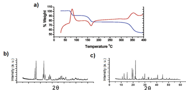
Fig. 20 (a) Thermogravimetric (blue trace) and DTA curves (red trace) of [\text{Cd}(\text{ADC})(\text{H}_2\text{O})_3]\cdot\text{H}_2\text{O} , (b) and (c) powder X-ray diffraction patterns of [\text{Cd}(\text{ADC})(\text{H}_2\text{O})_3]\cdot\text{H}_2\text{O} and [\text{Cd}(\text{ADC})(\text{H}_2\text{O})_{2.3}] , respectively. Reproduced from ref. 60 with permission of American Chemical Society, copyright 2003.
