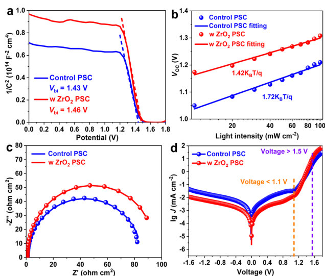
Fig. 3 (a) C - V curves, (b) dependence of V_{oc} on light intensity, (c) EIS spectra, and (d) dark J - V curves of control and ZrO_2 -capped CsPbI_2Br_2 PSCs.
