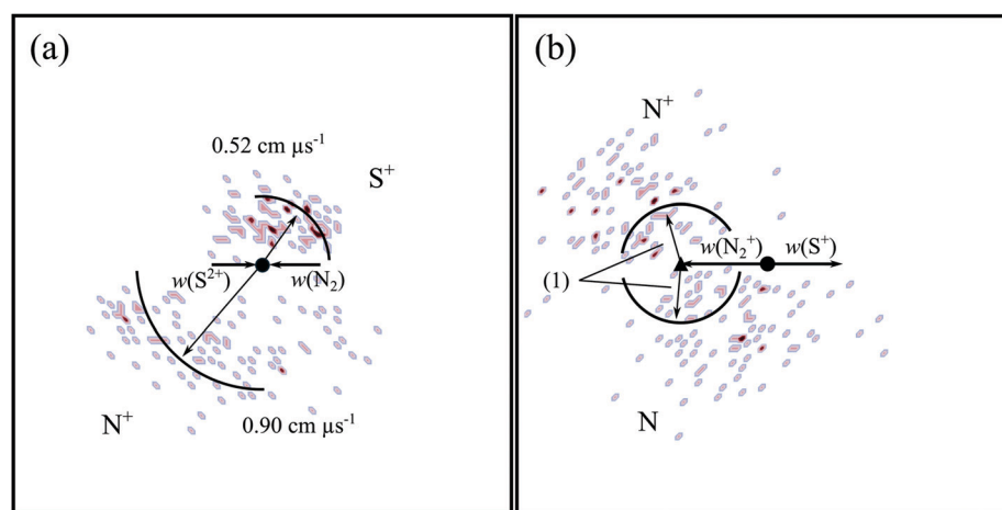
Fig. 11 Scattering diagrams for the DSET reaction S^{2+} + N_2 \rightarrow S^+ + N^+ + N at a CM collision energy of 4.7 eV. The black dot indicates the position of the CM. (a) CM scattering diagram showing the S^+ and N^+ products relative to the incident dication velocity, w(S^{2+}) . (b) Internal frame scattering diagram showing the scattering of N^+ and N relative to w(S^+) . In part (b) the labelled vector, (1), represents 0.44 \text{ cm } \mu\text{s}^{-1} .
