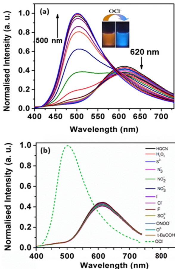
Fig. 4 (a) Fluorescence emission of HQCN (10 \mu M in \text{CH}_3\text{OH}-\text{H}_2\text{O} ; 1/4, v/v in the presence of HEPES buffer (10 mM) solution at pH = 7.2) upon the gradual addition of \text{OCl}^- (0 to 5 equivalents). Ratiometric spectra of HQCN were observed after the addition of \text{OCl}^- , where the \lambda excitation was 370 nm. The fluorescence emission peak at 620 nm gradually decreased and the peak at 500 nm gradually increased after the addition of \text{OCl}^- . Inset shows the visible emission of HQCN in the absence and presence of 2 equivalents of \text{HOCl} upon irradiation under UV light. (b) Fluorescence emission spectra of HQCN (10 \mu M in \text{CH}_3\text{OH}-\text{H}_2\text{O} ; 1/4, v/v in the presence of HEPES buffer (10 mM) solution at pH = 7.2) upon addition of different guest analytes (0 to 5 equivalents). Apart from \text{OCl}^- , no significant change was observed for other guest analytes.
