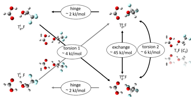
Fig. 7 Chirality-focused overview on the isomerisation options of the T_g complex at B3LYP-D3(BJ)/def2TZVP level (ZPE corrected). Facile hinge motion conserves the T_g chirality, whereas T_{g+} \leftrightarrow T_{g-} inversion can be achieved by alcohol torsion through a transition state with mirror plane or through an asymmetric transition state following hinge motion, and also by concerted double proton transfer through an exchange barrier above the OH stretching fundamental excitation.
