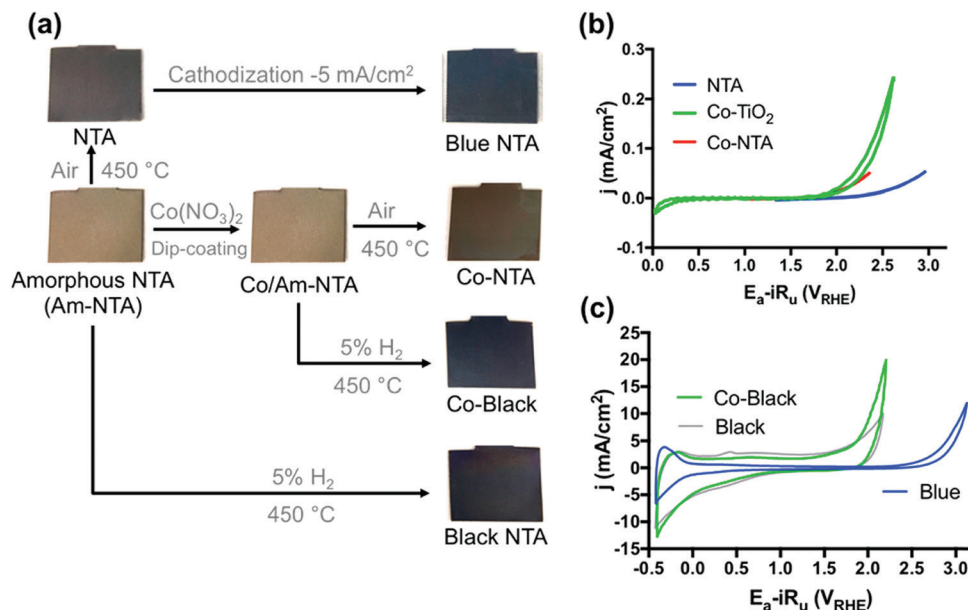
Fig. 28 NTA electrode preparation procedures. (b and c) Cyclic voltammograms of NTA electrodes in 100 \text{ mM KPi} buffer at pH 7.2. Reproduced with permission from ref. 539. Copyright American Chemical Society 2018.
