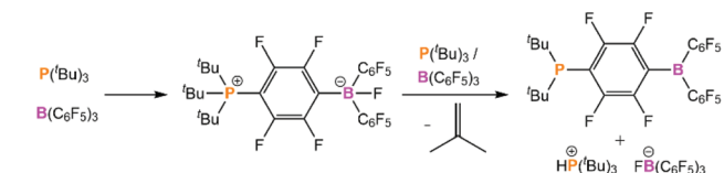
Scheme 2 Possible side-reaction between P(tBu)_3 and B(C_6F_5)_3 .
