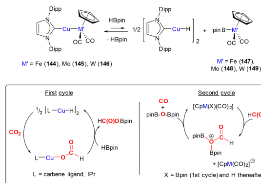
Scheme 43 Mechanism for the 2-electron reduction of \text{CO}_2 to CO catalysed by heterobimetallic complexes [(\text{NHC})\text{Cu--ML}_n] \{\text{ML}_n = [\text{FeCp}(\text{CO})_2], [\text{WCp}(\text{CO})_3], [\text{MoCp}(\text{CO})_3]\} .
