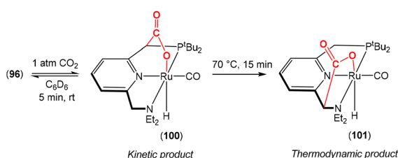
Scheme 32 Reactivity of CO 2 with dearomatized complex 96 and the formation of complexes 100 and 101 .
