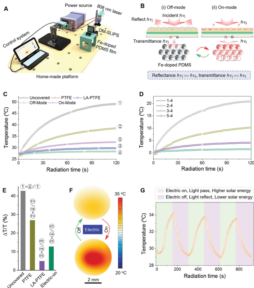
Fig. 5 Proof-of-concept for the DM-SLIPS shelter responsible for rational thermal management. (A) A homemade test system composed of a computer-controlled thermal IR imager, charging power source for triggering DM-SLIPS, 808 nm laser and Fe 3 O 4 -doped PDMS membrane. (B) The switching principle for realizing thermal management by selectively harvesting and reflecting solar irradiation depending on in situ charging/discharging of the DM-SLIPS shelter. With electricity on, a light release mode favorable for solar energy gain is achieved due to the intense photothermal effect. When the electricity is turned off, a light lock mode conducive to reflecting visible light back to the outer space is achieved. (C) Photothermal effect-induced temperature in terms of radiation time for air (uncovered), pristine PTFE, LA-PTFE, charging DM-SLIPS, and discharging DM-SLIPS shelters placed before the Fe 3 O 4 -doped PDMS membrane. (D) Temperature difference and (E) cooling amplitude of the Fe 3 O 4 -doped PDMS membrane sheltered by air (uncovered), pristine PTFE, LA-PTFE, and charged DM-SLIPS relative to that covered with discharged DM-SLIPS. (E) Thermal IR images and (F) temperature-time curve of the DM-SLIPS-sheltered Fe 3 O 4 -doped PDMS membrane in response to a cyclic electric trigger (6 V). The results show that the DM-SLIPS shelter exhibits a cooling temperature of 21.0 °C, superior to those of PTFE (10.6 °C) and LA-PTFE (19.4 °C). Significantly, this DM-SLIPS shelter is competent in reversibly switching the indoor temperature between 34 °C and 29 °C, thereby realizing selective solar energy gain/blockage.
