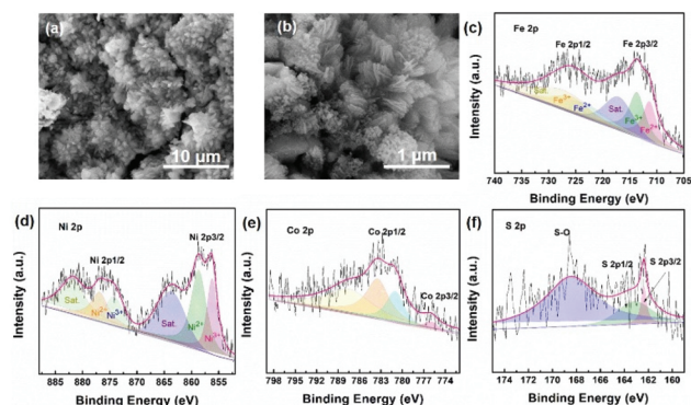
Fig. 4 SEM image (a) and (b), XPS survey spectra of Fe (c), Ni (d), Co (e) and S (f) of FeCoNi-NS-ACVs after a long-time stability test.
