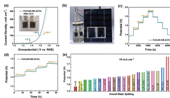
Fig. 5 (a) LSV curves of FeCoNi-NS-ACVs/F-FeCoP and the catalyst after 52 h stability test for overall water splitting in 1 M KOH (the inset is an image of the water splitting cell). (b) Solar cell driving overall water-splitting. (c and d) Stability tests of the obtained catalysts in 1 M KOH. (e) Comparison of the overpotentials (Ej10) with the references.
