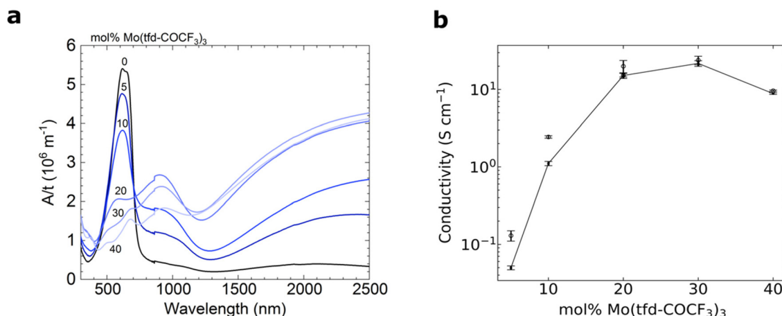
Fig. 5 (a) UV-Vis-NIR absorbance spectra with the measured absorbance A normalised by the film thickness t . (b) Electrical conductivity of 40–90 nm thick films of \text{p}(\text{g}_42\text{T-T}) doped with \text{Mo}(\text{tfd-COCF}_3)_3 ; average values and errors were obtained by measuring one sample for each dopant concentration five times and calculating the mean and standard deviation. The reproducibility of samples was confirmed by repeating the measurements on independently prepared films (Fig. S3† and open symbols in b).
