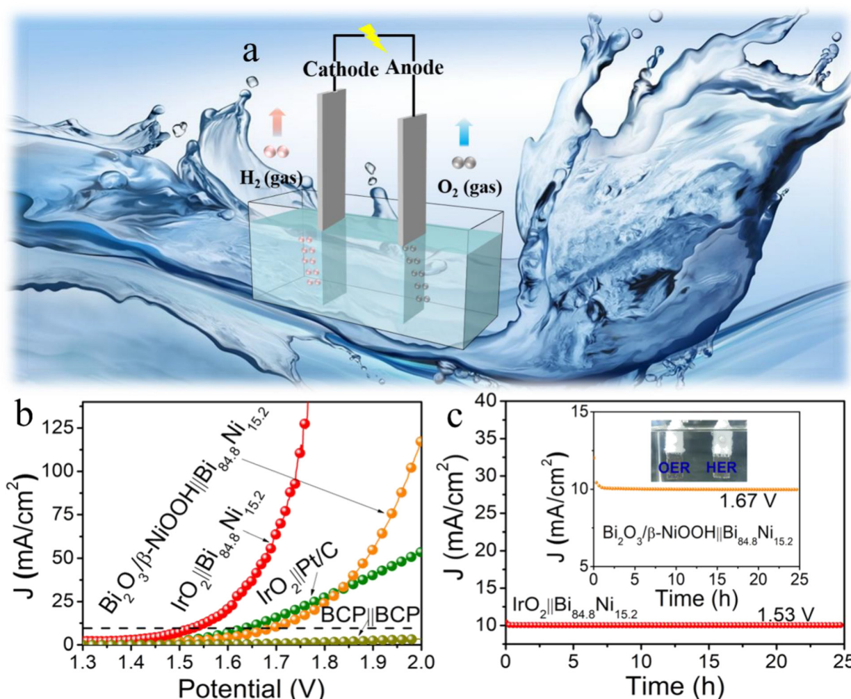
Fig. 5 Overall water splitting performance (a) two-electrode device; (b) polarization curves at a scan rate of 5\text{ mV s}^{-1} ; (c) I-t curves at an invariant cell voltage; Inset: image taken during water splitting.
