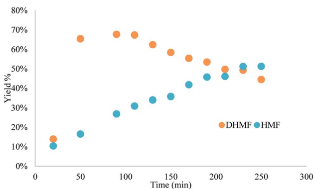
Fig. 8 Results of the scale-up reduction of HMF, with major decrease in catalytic activity. Reaction conditions: A 0.25 M solution of HMF in iso-propanol was pumped through a BZC column at 120^\circ\text{C} and 50 s residence time for 5.5 hours.
