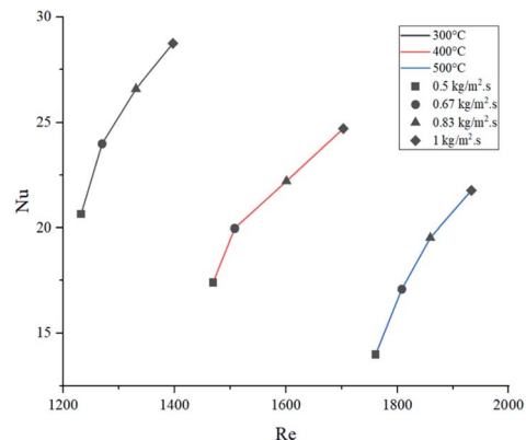
Fig. 11 Effect of Re on Nu at the operating conditions.
