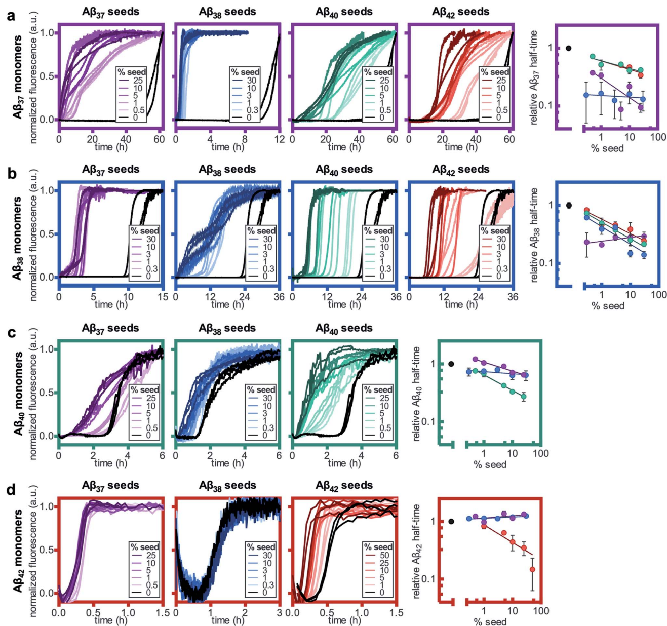
Fig. 8 Self- and cross-seeding experiments for monomeric (a) Aβ 37 , (b) Aβ 38 , (c) Aβ 40 , and (d) Aβ 42 . In all panels, the color of the frame corresponds to the identity of the monomeric peptide and the color of the kinetic curves corresponds to the identity of the seed peptide, with Aβ 37 , Aβ 38 , Aβ 40 , and Aβ 42 represented by purple, blue, green, and red, respectively. Seed concentrations are given as a molar percentage of the monomer concentration. The rightmost panel in each row shows the aggregation half-time as a function on seed percentage. Aβ 37 , Aβ 38 , and Aβ 40 monomer solutions were prepared to a peptide concentration of 10 μM, and Aβ 42 was prepared to a monomer concentration of 3 μM. All experiments were performed in 20 mM sodium phosphate buffer, pH 7.4, with 200 μM EDTA, 0.02% NaN 3 , and 20 μM ThT.
