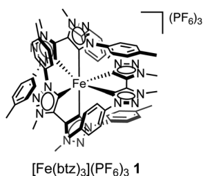
Fig. 1 Structure of the photoredox catalyst [Fe(btz) 3 ](PF 6 ) 3 1 used in this study.
