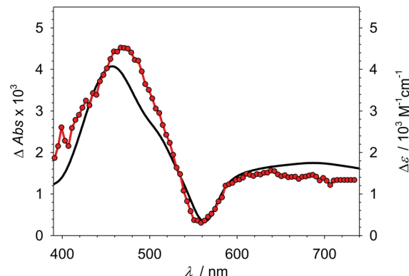
Fig. 2 Absorption changes upon laser flash excitation (490 nm) of [Fe(III)(btz) 3 ](PF 6 ) 3 1 in MeCN : MeOH (4 : 3) with TEA (0.29 M) (●) and difference spectrum between [Fe(III)(btz) 3 ](PF 6 ) 3 1 and [Fe(II)(btz) 3 ](PF 6 ) 2 2 (2-1, ▴).
