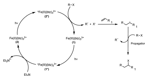
Scheme 3 Proposed reaction mechanism for the visible light-mediated ATRA reaction via reductive quenching of the excited state of [\text{Fe}(\text{btz})_3](\text{PF}_6)_3 1 .
