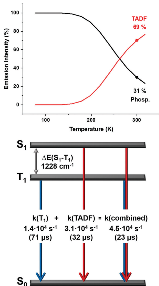
Fig. 9 Top: The emission intensities for complex 2 stemming from the singlet state S_1 (delayed fluorescence), and the triplet state T_1 (phosphorescence) as a function of the temperature according to eqn (3) and (4); bottom: a schematic energy level diagram and decay times of complex 2 in powder.
