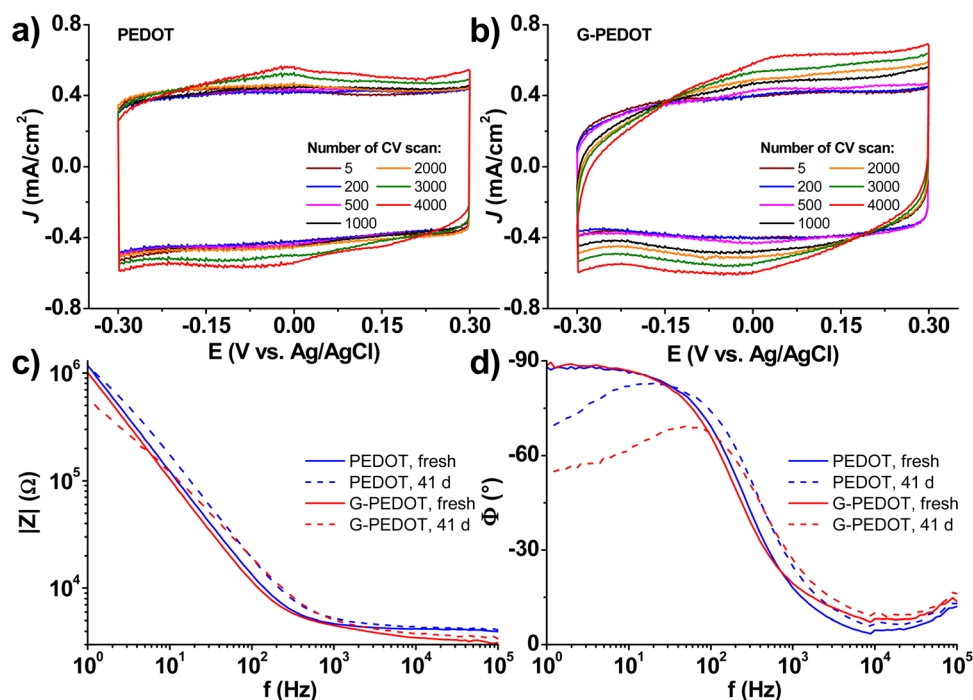
Fig. 4 Electrochemistry of PEDOT and G-PEDOT microelectrodes ( 50 \times 50 \mu\text{m} ) prepared by galvanostatic electropolymerization ( 2 \mu\text{C} : 20 \text{ nA} , 100 \text{ s} ) (a and b): selected cyclic voltammograms (scan rate = 100 \text{ mV s}^{-1} ) over 4000 cycles (electrochemical stability test); (c and d): electrochemical impedance spectra (bode plots, averaged over 2–3 different specimens) as prepared and after 41 days of accelerated aging test ( 60^\circ\text{C} , PBS solution).
