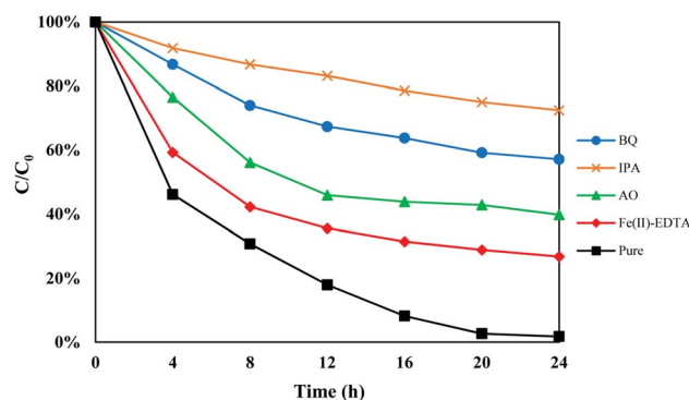
Fig. 10 Effect of radical scavengers on the POME degradation efficiency using the {001}- \text{TiO}_2/\text{Ti}_3\text{C}_2 aerogel composite.
