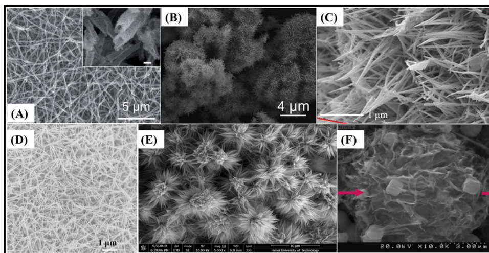
Fig. 5 SEM images of (A) hollow \text{ZnCo}_2\text{O}_4 nanotubes, 77 (B) urchin-like \text{ZnCo}_2\text{O}_4 microspheres, 64 (C) \text{ZnCo}_2\text{O}_4 nanorods/CC, 78 (D) \text{ZnCo}_2\text{O}_4 nanowire arrays/NF, 96 (E) porous \text{ZnCo}_2\text{O}_4 micro-urchins/NF 91 and (F) \text{ZnCo}_2\text{O}_4 intertwined heterostructured nanocubes/NF. 93 Panel A: Reproduced with permission. 77 Attribution 3.0 Unported (CC BY 3.0), Royal Society of Chemistry. Panel B: Reproduced with permission. 64 Copyright © 2018 Elsevier Ltd and Techna Group S.r.l. All rights reserved. Panel C: Reproduced with permission. 78 Copyright © 2018 Elsevier B.V. All rights reserved. Panel D: Reproduced with permission. 96 Panel E: Reproduced with permission. 91 Copyright © 2019, Springer-Verlag GmbH Germany, part of Springer Nature. Panel F: Reproduced with permission. 93 Copyright © 2019 Korean Physical Society. Published by Elsevier B.V. All rights reserved.
