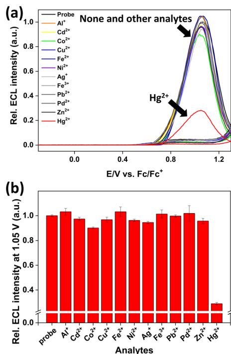
Fig. 6 (a) ECL intensities of probe 1 (10 \mu M) in the presence of various metal ions (40 \mu M each; \text{Hg}^{2+} 20 \mu M) in \text{CH}_3\text{CN}/\text{H}_2\text{O} (1:9 v/v, pH 7.4, 100 mM DBAE, 0.1 M HEPES, 0.1% polidocanol, and 0.1 M TBAP as the supporting electrolyte) while the potential is swept at a GC disk electrode (diameter 2 mm) in the range of -0.3 – 1.3 V (scan rate: 0.1 \text{ V s}^{-1} ). (b) ECL intensities at 1.05 V of probe 1 (10 \mu M) upon the respective addition of various metal ions (40 \mu M) and \text{Hg}^{2+} ions (20 \mu M).
