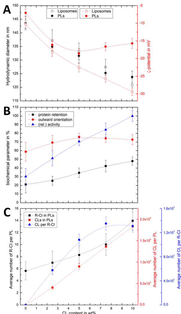
Fig. 3 Effect of CL on hydrodynamic diameter, \zeta -potential and biochemical competence of PLs, and average number of CL per PL and R-CL. (A) Change in hydrodynamic diameter (black) and \zeta -potential (red) with increasing CL content in PLs (1:50 protein:lipid ratio) and liposomes. (B) Biochemical parameters (protein retention, outward orientation, activity) against CL content. The activity, determined for a fixed amount of outward-facing R-CL of 1.5 \mu\text{g mL}^{-1} , is given as a relative value compared to the optimised system (DOPC:DOPE:CL 8:1:1). Data points represent mean values of two batches of PLs prepared with increasing CL content. (C) Effect of increasing CL content on the average number of R-CL in PLs with protein:lipid ratio 1:50 (black), with number of CL units in PLs (red) and the average number of CLs per reconstituted R-CL (blue). Dashed lines serve as a guide to the observed trends.
