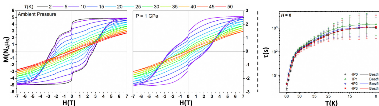
Fig. 2 Hysteresis loops of 1 at 2 K and 5–50 K in 5 K steps recorded at ambient pressure (left) and at 1 GPa (centre). For the series at 1 GPa, data below \pm 800 Oe at 5 K are omitted due to the superconductive manometer (Pb). Right: Relaxation profile ( \tau vs. T ) for 1 at ambient pressure (HP0), 0.37 GPa (HP1), 0.79 GPa (HP2) and 1.2 GPa (HP3) (see Fig. S41 and S42, ESI† for fitted data and variations in the distribution of \tau ( \beta ) with temperature).
