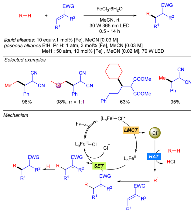
Scheme 7 Iron-catalysed functionalization of alkenes enabled by LCMT \text{Cl}^\bullet generation.
