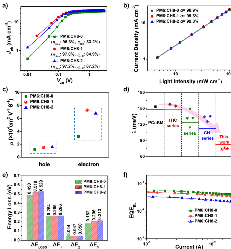
Fig. 3 (a) Plots of J_{ph} versus V_{eff} . (b) Dependence of current density ( J_{sc} ) on P_{light} of optimized OSCs. (c) Hole and electron mobilities of PM6:CH8-0, PM6:CH8-1 and PM6:CH8-2 based devices. (d) A summary of the electron reorganization energy of several representative series of electron acceptors. (e) Detailed E_{loss} of CH8-0, CH8-1 and CH8-2 based devices. (f) EQE EL spectra of PM6:CH8-0, PM6:CH8-1 and PM6:CH8-2 based OSCs; EQE EL values for CH8-0, CH8-1 and CH8-2 based devices are 5.15 \times 10^{-4} , 4.55 \times 10^{-4} and 3.24 \times 10^{-4} , respectively.
