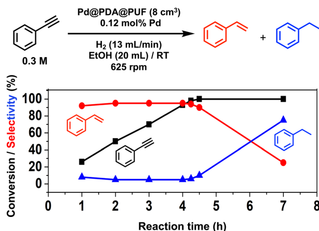
Fig. 5 Hydrogenation of phenylacetylene with Pd@PDA@PUF (8 \text{cm}^3 ); EB selectivity. Reaction conditions: PA (6 mmol), Pd (7 \times 10^{-3} mmol, 0.12 mol%), EtOH (20 mL), \text{H}_2 flow rate (13 \text{mL min}^{-1} ), room temperature, 625 rpm.
