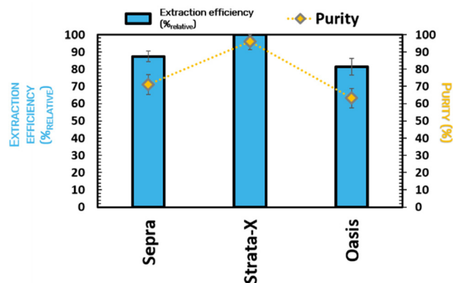
Fig. 7 Extraction efficiency (%relative) and purity rate (%) of anthocyanins from Jabuticaba wastes with different adsorbent materials (Septra \text{C}_{18} -E, Strata-X \text{C}_{18} , and Oasis HBL \text{C}_{18} ) in the SPE step.
