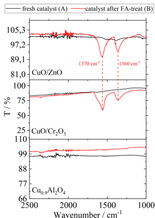
Fig. 4 ATR-IR spectra of CuO/ZnO, CuO/Cr 2 O 3 and \text{Cu}_{0.9}\text{Al}_{2.0}\text{O}_4 before (A) and after (B) contact with FA; assignment of peaks: carboxylate ion of formate species (1570 cm -1 asymmetric stretch and 1360 cm -1 symmetric stretch). 33
