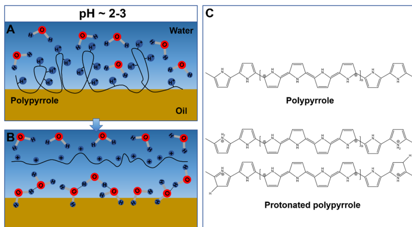
Scheme 3 pH-dependent adsorption and desorption of polypyrrole at the oil–water interface. Polypyrrole is firstly protonated by the protons ( \text{H}^+ ) at pH \sim 2 –3 (A), and subsequently adopts an extended conformation as a result of the electrostatic interaction, and desorbs from the oil–water interface due to a reduction in free energy (B). (C) The chemical structures of the pristine polypyrrole and protonated polypyrrole.
