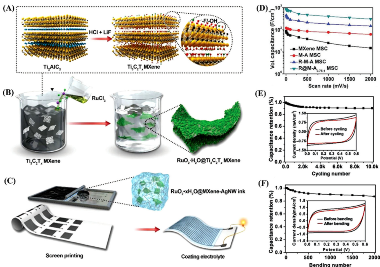
Fig. 7 Illustration of (a) the preparation of \text{Ti}_3\text{C}_2\text{T}_x MXenes; (b) procedure for the synthesis of the \text{RuO}_2 \cdot x\text{H}_2\text{O}@\text{MXene} nanocomposite; (c) development of flexible MSC devices through screen printing; a graphical image showing (d) the volumetric capacitance of various MXene MSCs at diverse scan rates; (e) plot of cycling stability at 100 \text{ mV s}^{-1} (inset: CV curves recorded before and after cycling); and (f) plot of cycling stability with a bending strain of 5.0% at various bending cycles (the inset shows CV curves recorded before and after 2000 bending cycles at 100 \text{ mV s}^{-1} ). 108 Reproduced from ref. 108 with permission from Wiley-VCH, copyright 2019.
