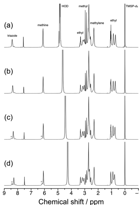
Fig. 6 ^1\text{H} NMR spectra for a 1.0 wt% solution of syndio -poly(ME)-3 in \text{D}_2\text{O} measured at 20 (a), 40 (b), 60 (c), and 80 ^\circ\text{C} (d).
