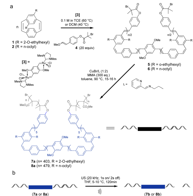
Scheme 1 Synthesis (a) and mechanical activation (b) of coil-rod-coil ABA phenylene-vinylene triblock copolymers 7a and 8a .
