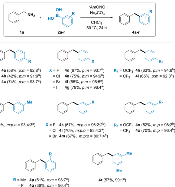
Fig. 3 Arylboronic acid scope of the deaminative coupling between benzylamines and arylboronic acids. Reaction conditions: benzylamine ( 1a , 2.0 mmol), arylboronic acid ( 2a–r , 0.5 mmol), isoamyl nitrite (2.5 mmol), sodium carbonate (0.5 mmol), chloroform (1.25 mL), 60 °C, 24 h. Isolated yields after flash column chromatography. a Isomer ratio determined by 13 C NMR. b Isomer ratio determined by 19 F NMR.
