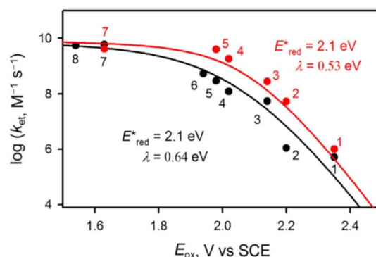
Fig. 4 Plots of \log k_{et} of electron transfer from electron donors [(1) \text{C}_6\text{H}_6 , (2) \text{PhCH}_3 , (3) \text{PhCH}_2\text{CH}_3 , (4) m -xylene, (5) mesitylene, (6) \text{PhCH}_2\text{OH} , (7) durene, and (8) naphthalene] to \{[(\text{BnTPEN})\text{Mn}^{\text{IV}}(\text{O})]^{2+}\text{-(Sc}(\text{NO}_3)_3)_2\}^* (red circles) and [(\text{BnTPEN})\text{Mn}^{\text{IV}}(\text{O})]^{2+}\text{-(Sc}(\text{OTf})_3)_2 (black circles) against E_{ox} values of electron donors in TFE/MeCN (v/v 1 : 1) at 298 K. Reprinted from ref. 61 with permission from John Wiley and Sons (Copyright 2020).
