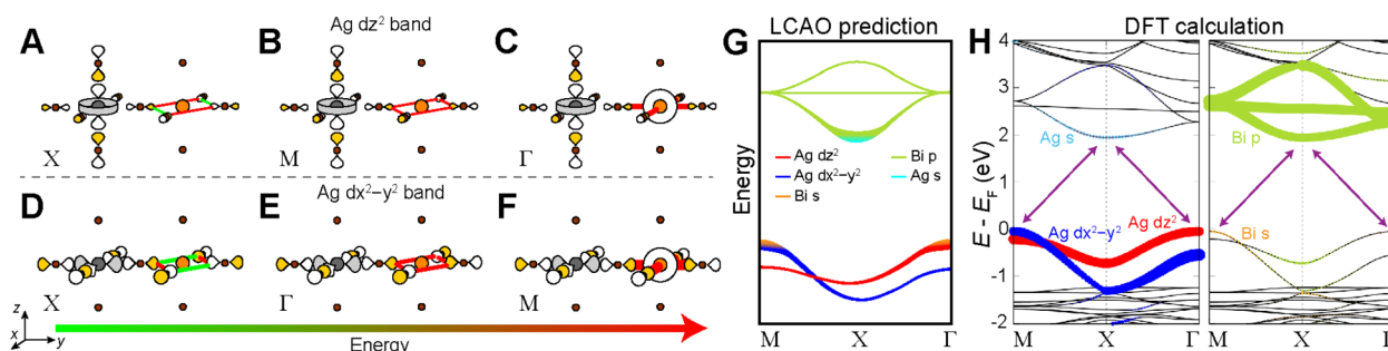
Fig. 8 LCAO analysis for the n = 1 Ag–Bi structure. LCAO representations of the Ag \text{d}_{z^2} derived valence band (VB) at the X (A), M (B), and \Gamma (C) points ranked in order of increasing energy from left to right. LCAO representations of the Ag \text{d}_{x^2-y^2} derived VB at the X (D), \Gamma (E), and M (F) points ranked in order of increasing energy from left to right. Bonding and antibonding interactions at the \text{B}' site are shown as green and red lines, respectively, and the thickness of each line corresponds to the strength of the interaction. Halide p orbital lobes are scaled to represent approximate relative electron densities and the shading of orbital lobes denote their relative phases. Gray, orange, and brown spheres represent Ag, Bi, and Br atoms, respectively. (G) Predicted band diagram of the n = 1 Ag–Bi structure using our LCAO analysis. (H) DFT band structure of the n = 1 Ag–Bi structure without SOC. The band structure is shown in duplicate where the Ag (left panel) and Bi (right panel) states that compose the bands are represented by colored dots.
