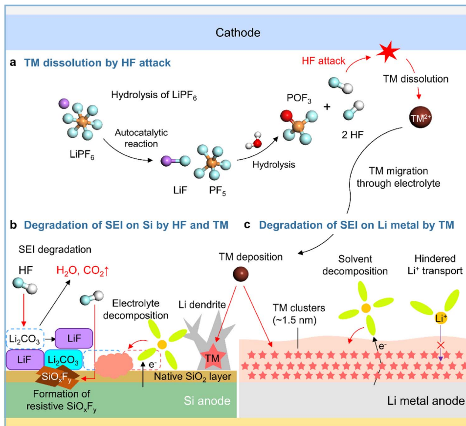
Fig. 5 Schematic illustration of (a) LiPF 6 hydrolysis and HF-triggered transition metal (TM) dissolution from the cathode, (b) degradation of the SEI on the silicon anode caused by HF attack and TM deposition, and (c) degradation of the SEI on the lithium-metal anode caused by TM deposition.
