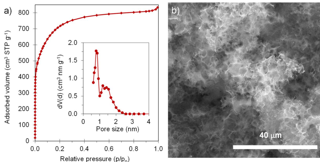
Fig. 4 (a) \text{N}_2 adsorption isotherm (inset: QSDFT PSD) and (b) SEM micrograph of AGA-850.
