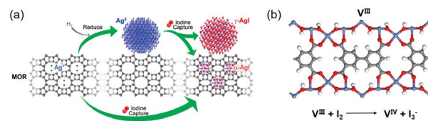
Fig. 2 (a) Schematic of the I 2 capture process using Ag-MOR zeolite as the adsorbent. For Ag 0 sites, I 2 adsorption leads to the formation of two AgI phases, i.e. , α-AgI clusters in the zeolite pores and γ-AgI nanoparticles on the zeolite surface. For Ag + sites, only α-AgI clusters are formed in the pores. Reproduced with permission from ref. 34. Copyright 2010, American Chemical Society. (b) Structure model of MOF MFM-300(VIII) and the redox reaction upon I 2 adsorption. Color code: blue, V III ; red, O; gray, C; white, H. 43
