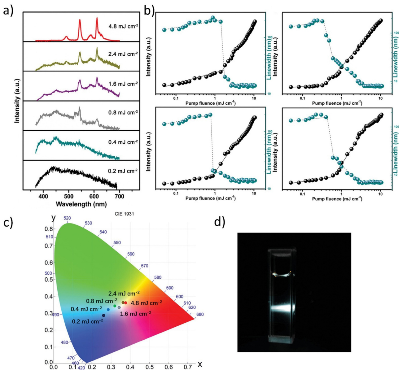
Fig. 11 (a) Emission spectra from the V 2 C MQD colloid for different pump fluences. (b) Dependence of peak intensity and linewidth of the dominant emission peaks plotted as a function of pump fluences shows the lasing threshold behavior. (c) The plot of the calculated CIE coordinates of emission spectra under different pumping fluence (0.2 mJ cm -2 (0.269, 0.294); 0.4 mJ cm -2 (0.296, 0.325); 0.8 mJ cm -2 (0.329, 0.34); 1.6 mJ cm -2 (0.349, 0.334); 2.4 mJ cm -2 (0.373, 0.365); 4.8 mJ cm -2 (0.383, 0.365)). (d) Photos of the operating V 2 C MQDs colloid under 355 nm pulsed laser pumping at 4.8 mJ cm -2 . Reproduced or Adapted with permission. 16 2019, Wiley.
