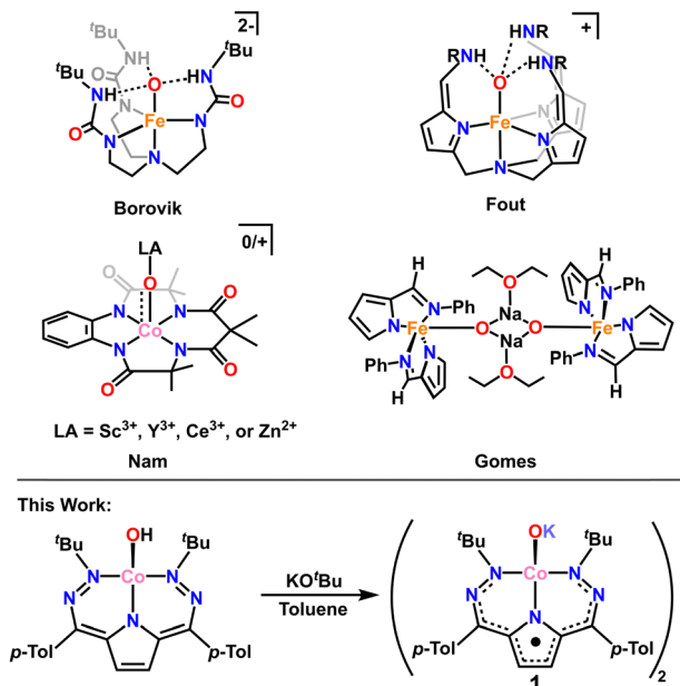
Scheme 1 Top: Examples of previously reported metal oxides stabilized by hydrogen bonding or Lewis acid interactions. Bottom: Synthesis of 1 from [\text{t}^{\text{Bu,Tol}}\text{DHP}]\text{CoOH} .
