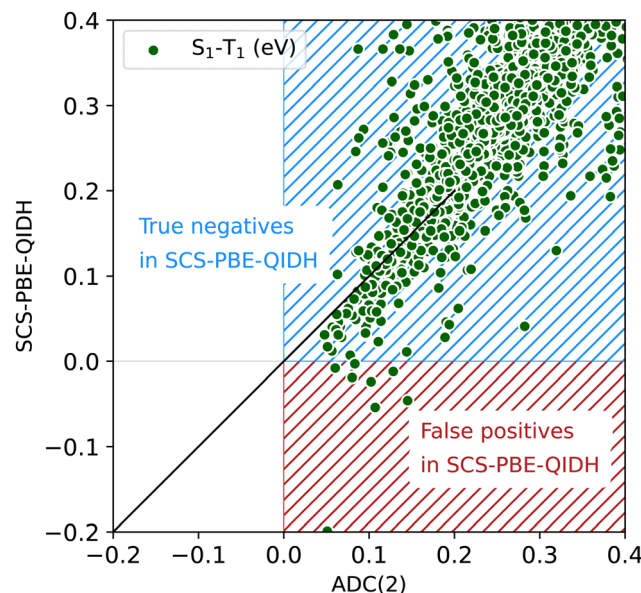
Fig. 4 Scatterplot of S_1-T_1 energy gap \leq 0.4 eV from SCS-PBE-QIDH and ADC(2) for the bigQM70 molecules.
