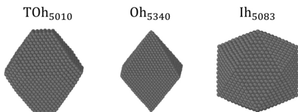
Fig. 3 Snapshots of the different NP shapes studied in the present work: truncated octahedron (TOh), octahedron (Oh) and icosahedron (Ih). Particles of similar sizes are displayed, but a wide range of sizes is covered.
